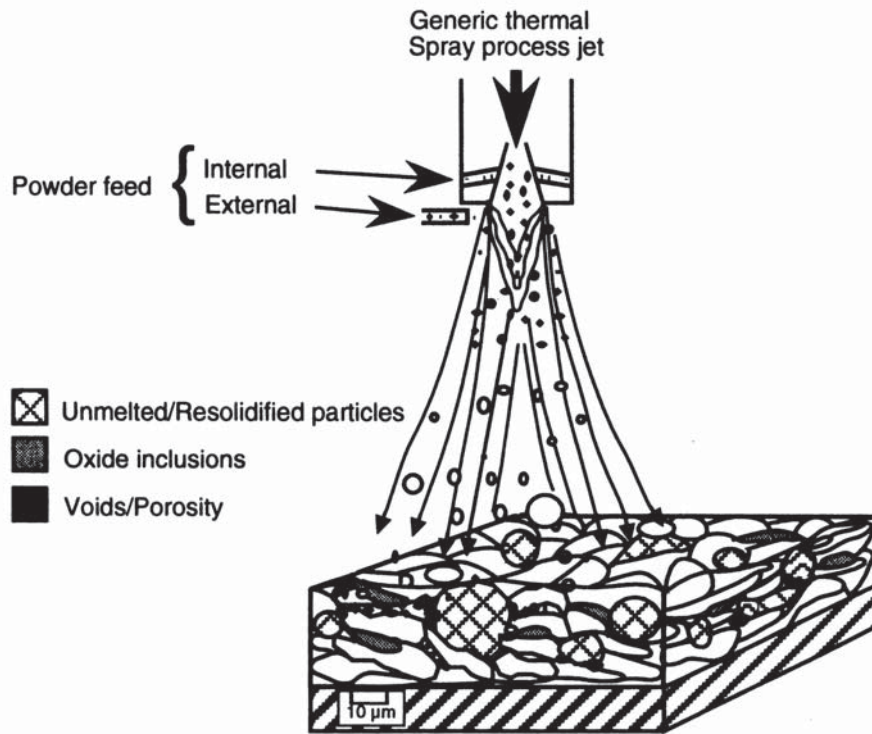
Schematic of a typical thermal-spray powder process. Source: J.R. Davis (Ed.), Handbook of Thermal Spray Technology , ASM International, p 4, 2004
