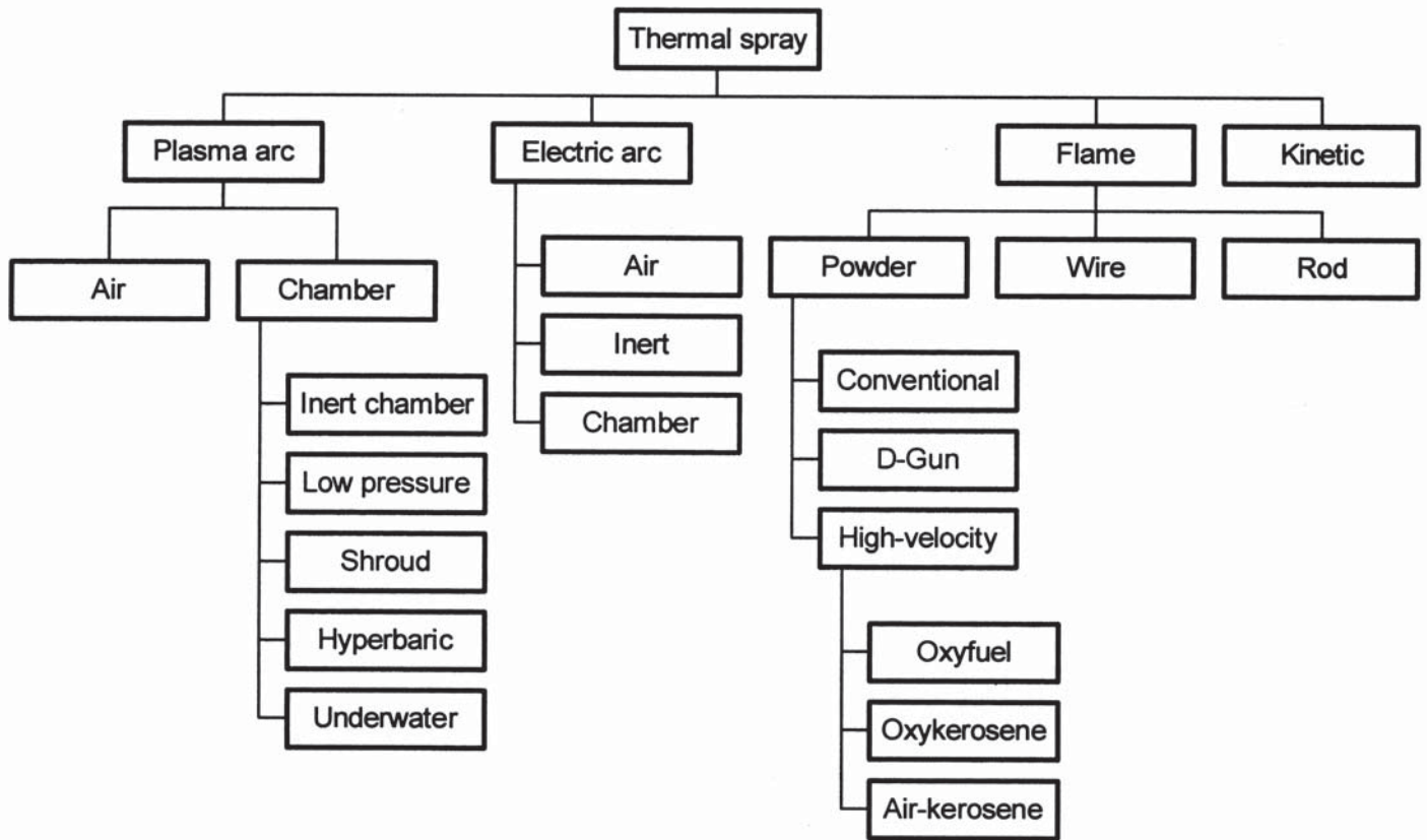
Thermal spray processes and subsets. Source: J.R. Davis (Ed.), Handbook of Thermal Spray Technology , ASM International, 2004, p 44
