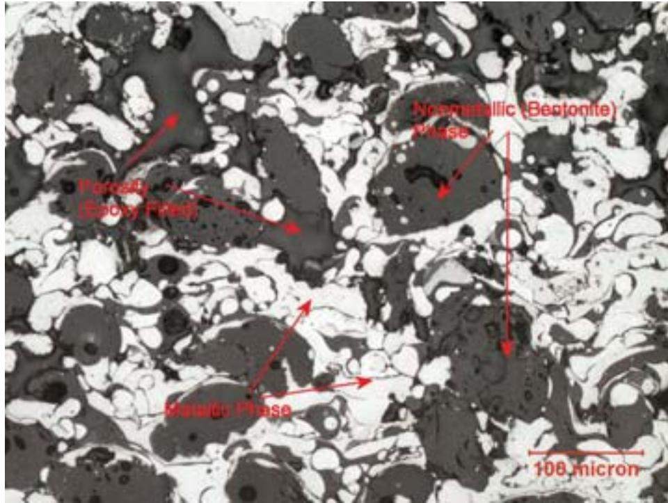
Typical microstructure for Ni-4Cr-4Al/Bentonite
