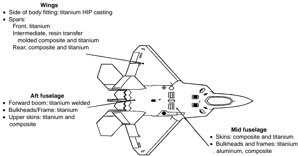
Fig. 2.5 Some areas of titanium use in the F-22 Raptor advanced fighter aircraft
